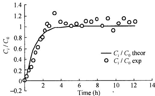
Fig. 4. Calculated versus measured time-course of lactate concentration in the construct centre.
