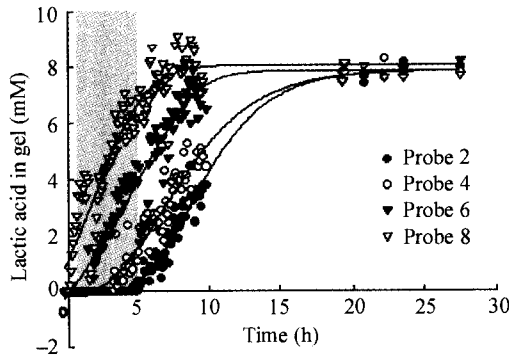
Fig. 3. The time-course of lactate concentrations in the gel measured at four probes (for clarity), with probe 2 closest to the perfusing surface and probe 8 farthest from it. Results in shadow were used for estimation of solute diffusivity.
